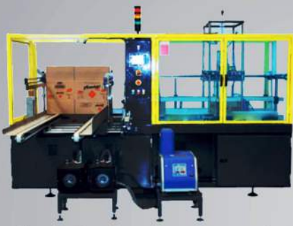
Case Erector 3000 series Upto 40 Cases/min
